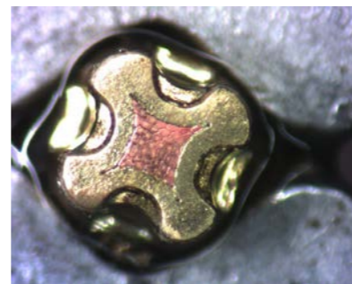
4/8-indent crimp
